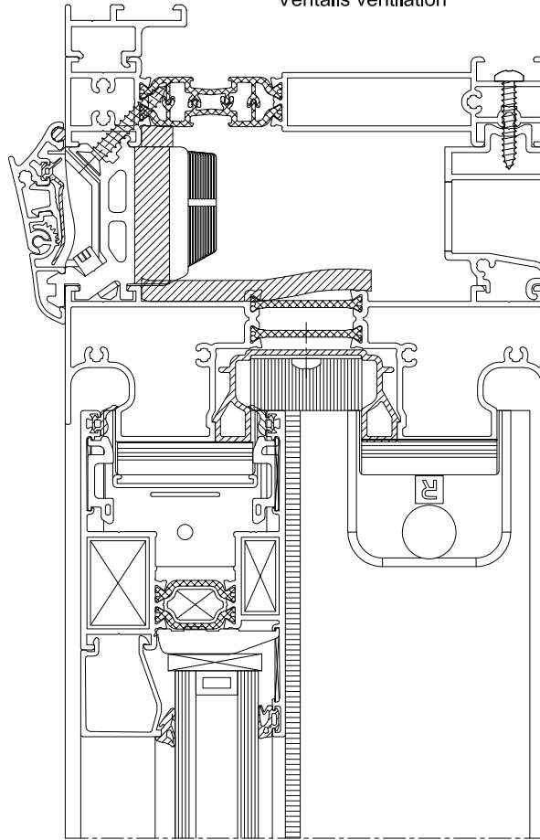
Ventalis ventilation
